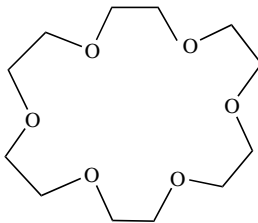
Figure 1.2 [18]-crown-6 ether.
