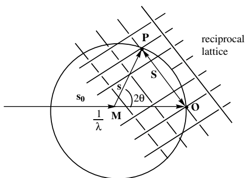
Figure 3.7 The Ewald sphere used to construct the direction of the scattered beam. The sphere has radius 1/\lambda . The origin of the reciprocal lattice is O . The incident X-ray beam is labeled s_0 and the scattered beam is labeled s . (Adapted with permission from Figure 4.19 of Drenth, J. Principles of Protein X-Ray Crystallography , 2nd ed., Springer-Verlag, New York, 1999. Copyright 1999, Springer-Verlag, New York.)
