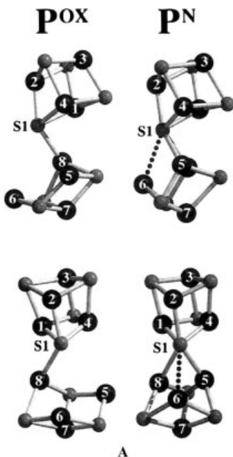
Figure 6.7 (A) Structural models of P N and P OX as reprinted from Figure 2 of reference 24. (B) Comparison of P N and P OX structures as reprinted from Figure 4 of reference 24. (Both figures reprinted with permission from Peters, J. W.; Stowell, M. H. B.; Soltis, S. M.; Finnegan, M. G.; Johnson, M. K.; Rees, D. C. Biochemistry 1997, 36 , 1181–1187. Copyright 1997, American Chemical Society.)
